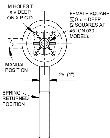
ISO MOUNT
