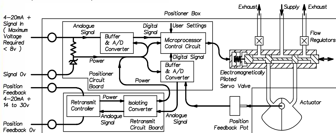
Simplified Functional Diagram of EL Positioner
