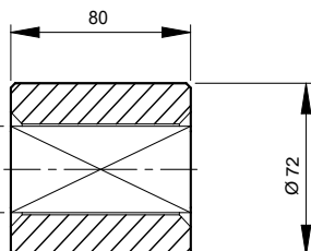
Standard Coupling (supplied with actuator weight 3.7 lbs/1.7 kg)
