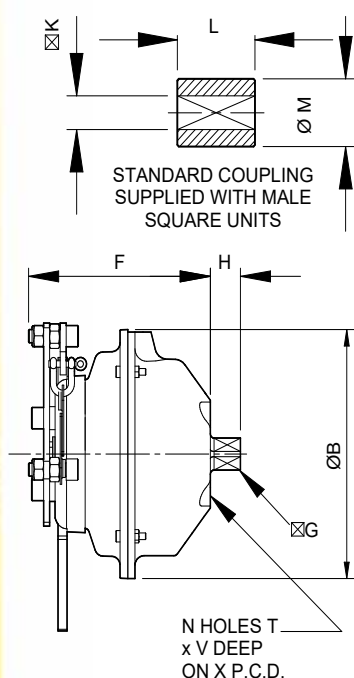
Model 05 & 07
