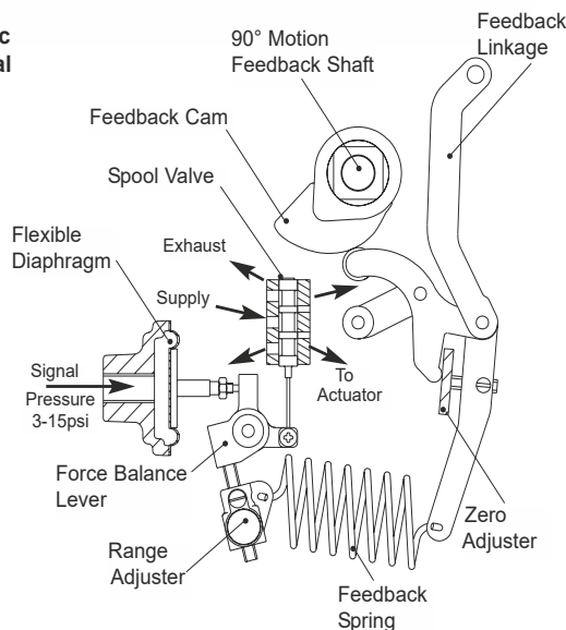
Schematic Functional Diagram
