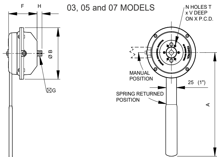
ISO MOUNT
