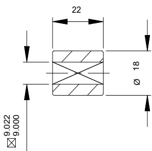
Standard Coupling (supplied with actuator weight 0.07 lbs/0.03 kg)
