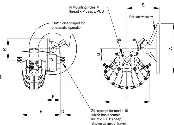
DRAWING SHOWS RIGHT HAND HANDWHEEL.
