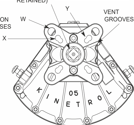
FEMALE BI-SQUARE G x E DEEP (COUPLING RETAINED)
